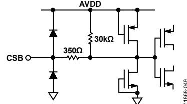
Figure 43. Equivalent CSB Input Circuit
