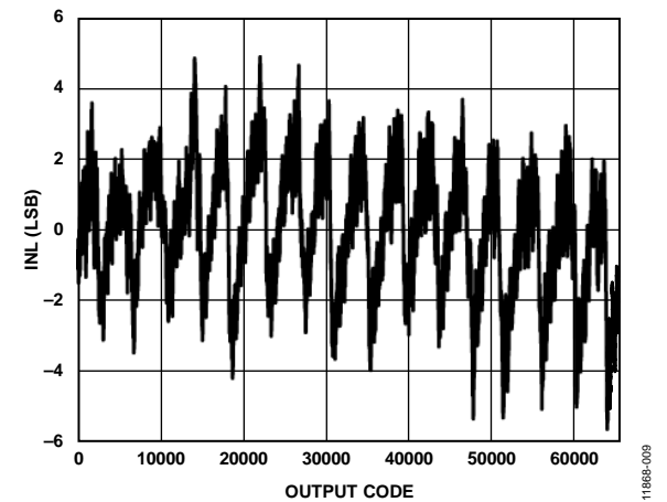
Figure 32. Integral Nonlinearity (INL), f_{IN} = 9.7 MHz, f_{SAMPLE} = 125 MSPS, V_{REF} = 1.0 V
