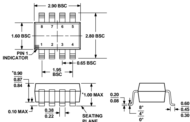
*COMPLIANT TO JEDEC STANDARDS MO-193-BA WITH THE EXCEPTION OF PACKAGE HEIGHT AND THICKNESS. Figure 48. 8-Lead Small Outline Transistor Package [TSOT] (UJ-8)
