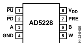
Figure 6. SOT-23-8 Pin Configuration
