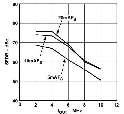
Figure 8. SFDR vs. f_{OUT} and I_{OUTFS} @ 25 MSPS and 0 dBFS
