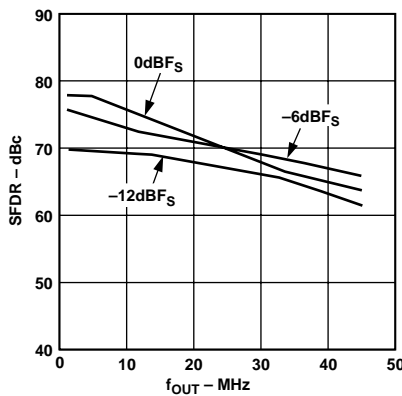
Figure 6. SFDR vs. f_{OUT} @ 100 MSPS
