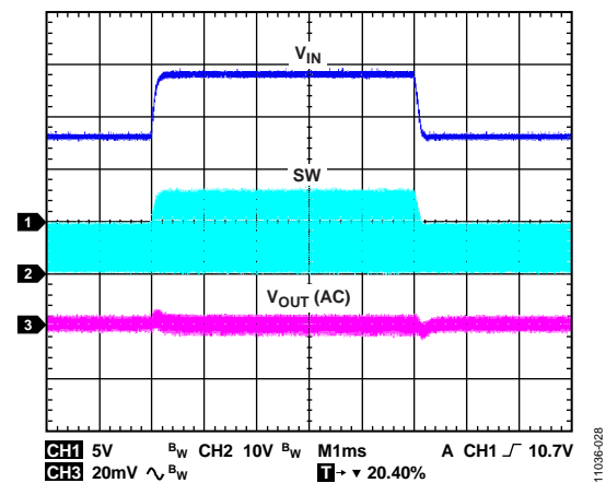
Figure 28. Line Transient Response, V_{IN} from 8 V to 14 V, I_{OUT} = 1 A
