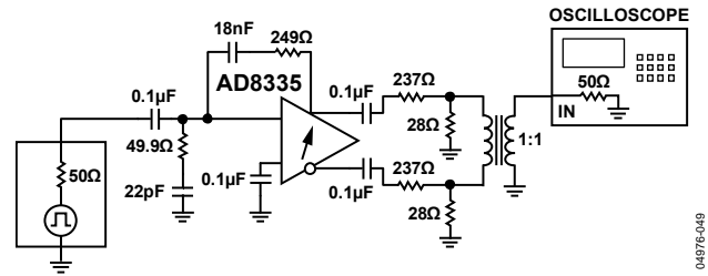
Figure 51. Test Circuit for Transient Measurements
