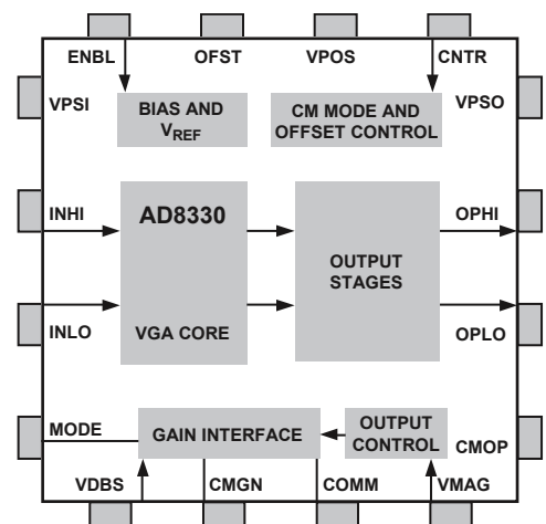
Figure 46. Block Schematic
