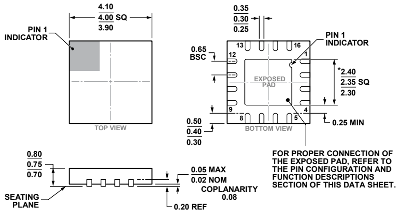
Figure 49. 16-Lead Lead Frame Chip Scale Package [LFCSPP] 4 mm x 4 mm Body and 0.75 mm Package Height (CP-16-20) Dimensions shown in millimeters
