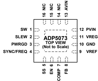
Figure 2. Pin Configuration
