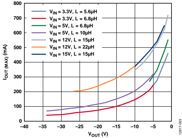
Figure 3. Maximum Output Current, f_{SW} = 1.2 \text{ MHz} , T_A = 25^\circ\text{C} , Based on Target of 70% I_{LIM(MIN)}
