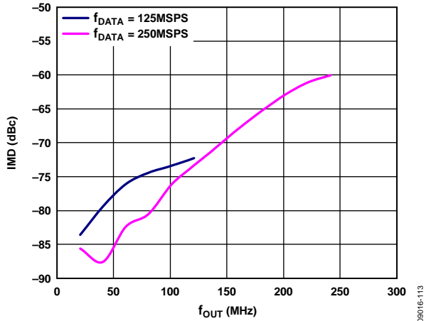
Figure 16. IMD vs. f_{OUT} over f_{DATA} , 2× Interpolation, Digital Scale = 0 dBFS, f_{SC} = 20 mA
