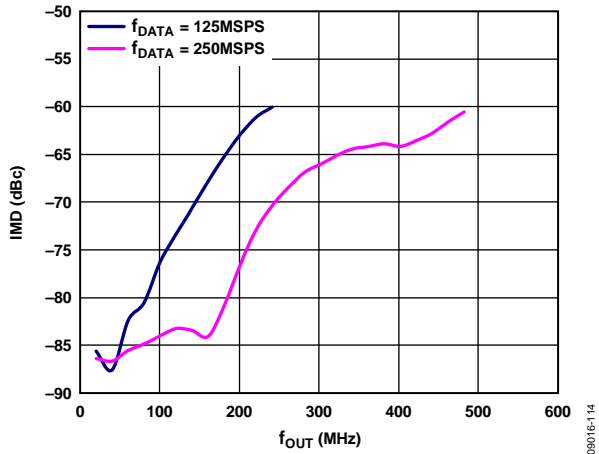
Figure 17. IMD vs. f_{OUT} over f_{DATA} , 4× Interpolation, Digital Scale = 0 dBFS, f_{SC} = 20 mA
