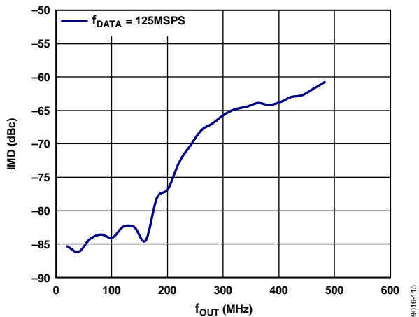
Figure 18. IMD vs. f_{OUT} over f_{DATA} , 8× Interpolation, Digital Scale = 0 dBFS, f_{SC} = 20 mA
