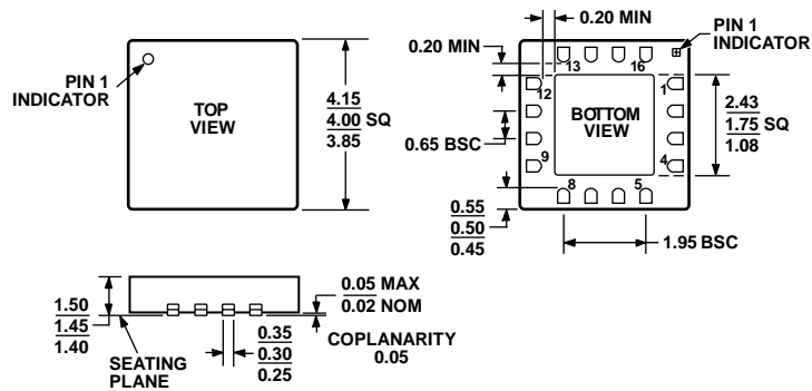
Figure 21. 16-Lead Lead Frame Chip Scale Package [LFCSP_LQ] 4 mm x 4 mm Body (CP-16-5a*) Dimensions shown in millimeters
