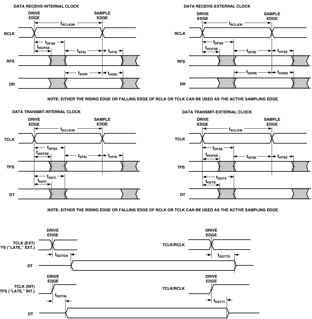
Figure 18. Serial Ports
