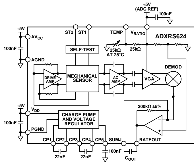
Figure 1. ADXRS624 Block Diagram
