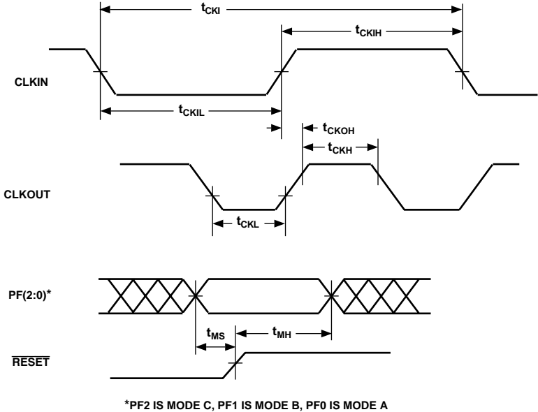
Figure 8. Clock Signals
