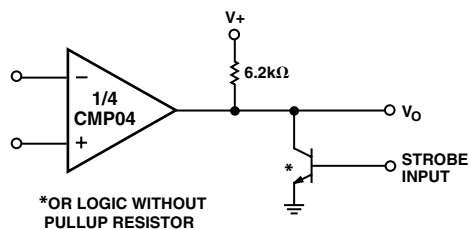
Figure 4. Output Strobging
