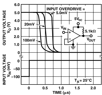
TPC 7. Response Time for Various Input Overdrives—Negative Transition
