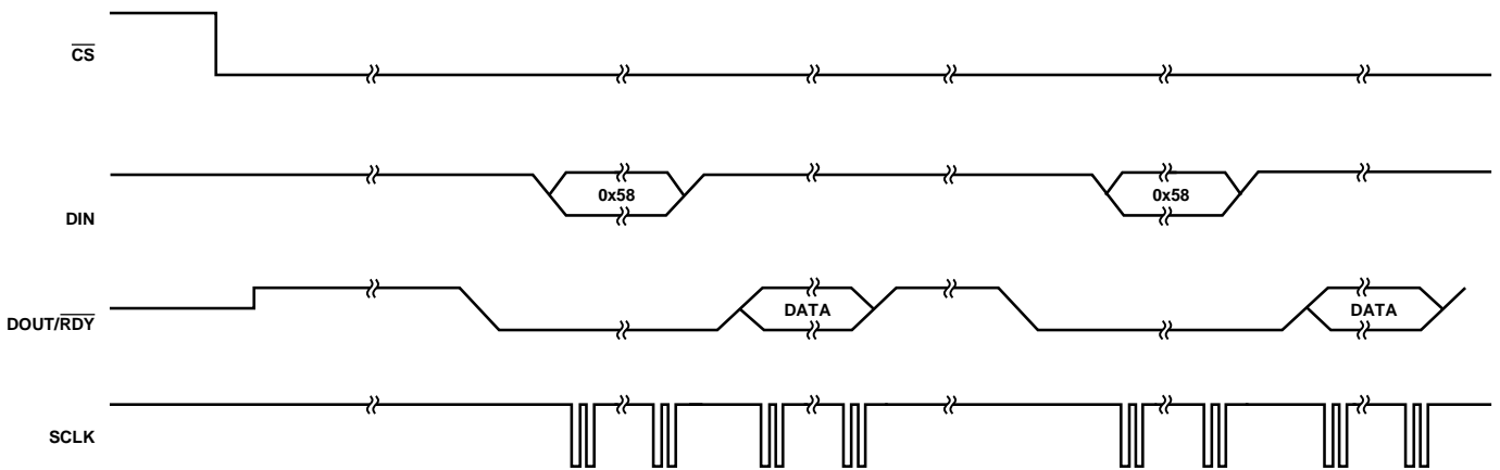
Figure 22. Continuous Conversion
