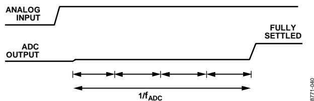
Figure 27. \text{Sinc}^4 Zero Latency Operation
