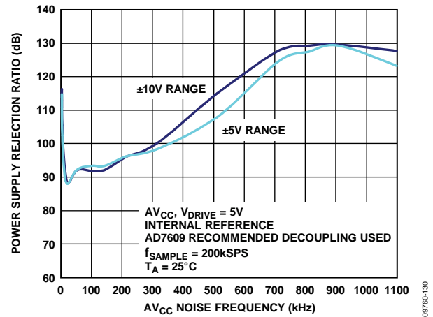
Figure 30. PSRR
