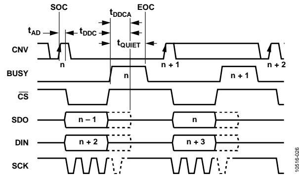
Figure 70. Data Access During Conversion
