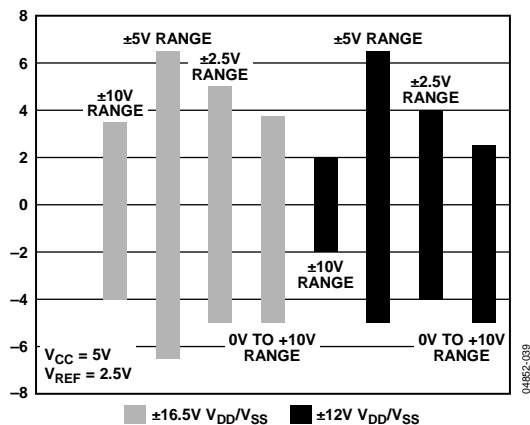
Figure 40. Pseudo Differential Input Range with V_{CC} = 5\text{ V}
