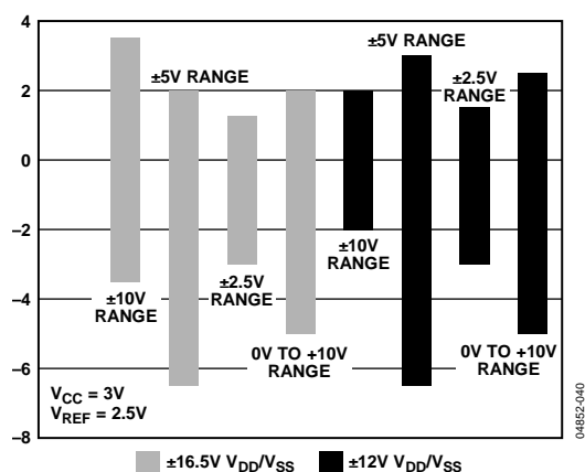
Figure 41. Pseudo Differential Input Range with V_{CC} = 3\text{ V}
