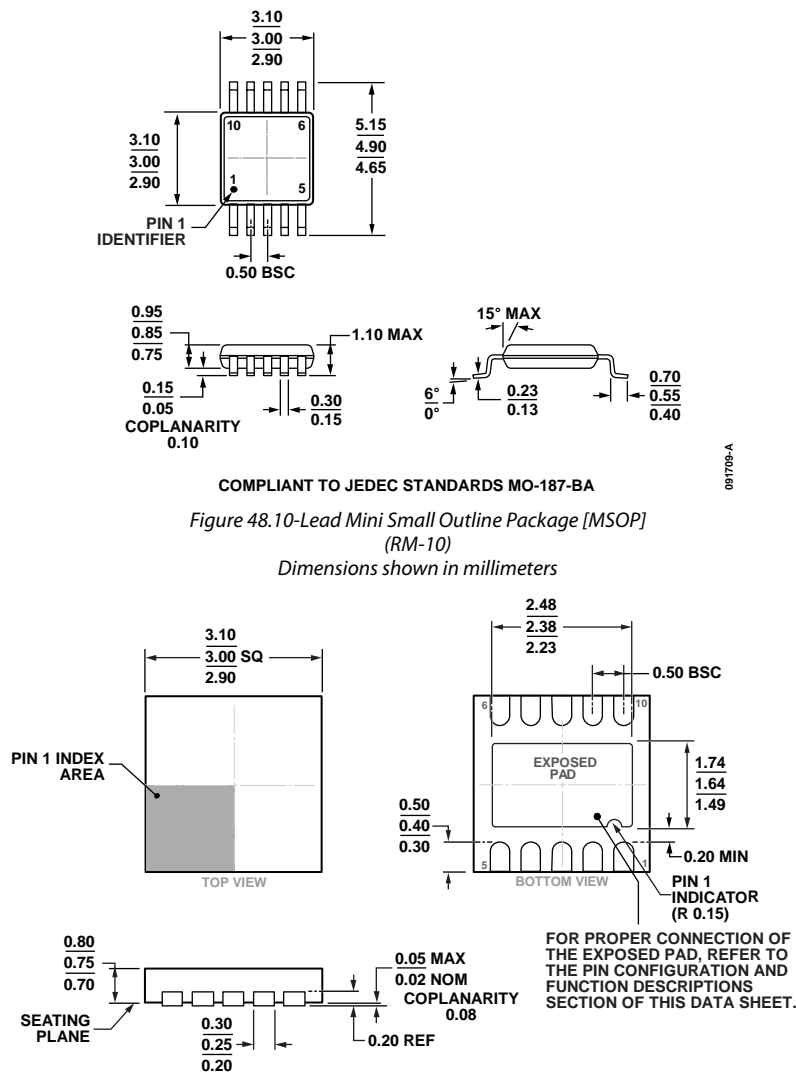
Figure 49. 10-Lead Lead Frame Chip Scale Package [LFCSP_WD] 3 mm × 3 mm Body, Very Very Thin, Dual Lead (CP-10-9)
