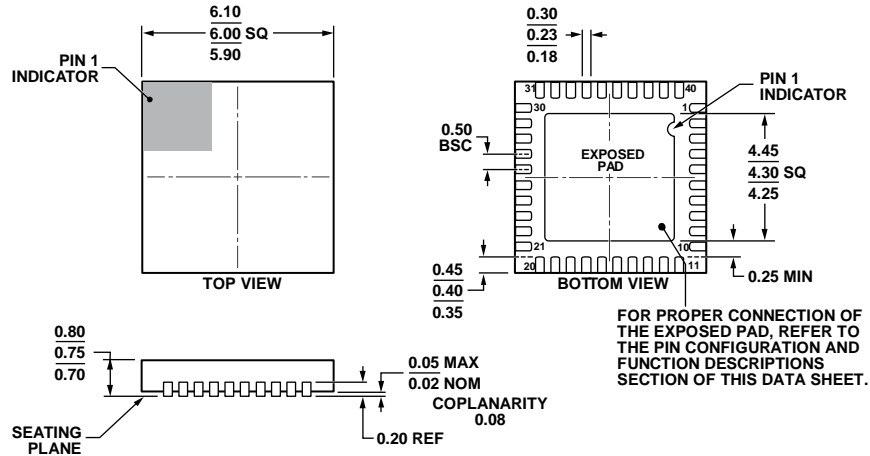
Figure 40. 40-Lead Lead Free Chip Scale Package [LFCSP_WQ] 6 mm x 6 mm Body, Very Very Thin Quad (CP-40-10) Dimensions shown in millimeters
