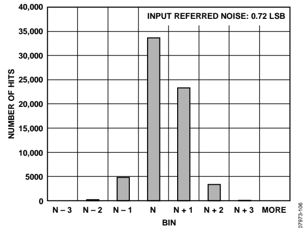
Figure 21. Input-Referred Noise Histogram, f_{SAMPLE} = 170 MSPS
