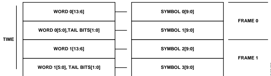
Figure 64. AD9644 14-Bit Data Transmission with Tail Bits
