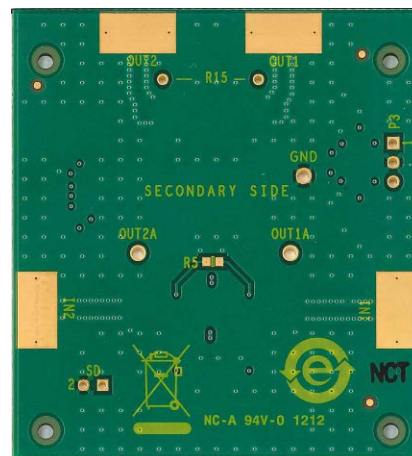
Figure 20. Evaluation Board Bottom Layer
