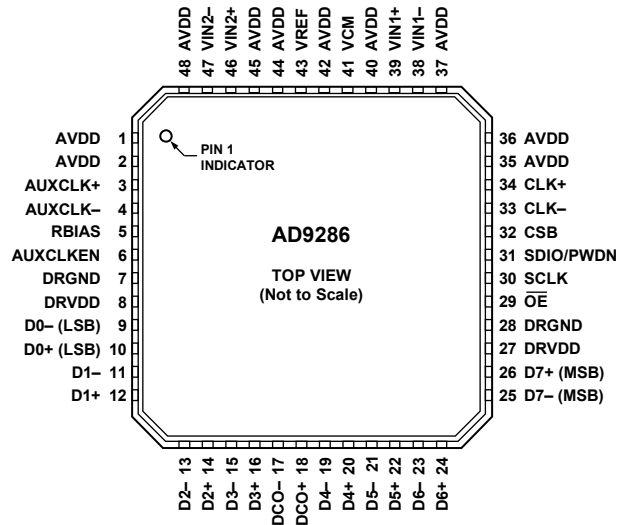
Figure 6. Pin Configuration
