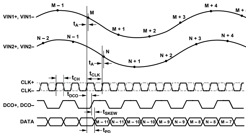
Figure 2. Output Timing Diagram, Sample Mode = Interleaved (Default)
