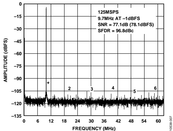
Figure 7. Single-Tone 16k FFT with f_{IN} = 9.7\text{ MHz} , f_{SAMPLE} = 125\text{ MSPS} , V_{REF} = 1.0\text{ V}
