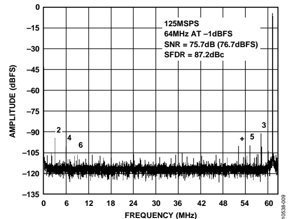
Figure 9. Single-Tone 16k FFT with f_{IN} = 64\text{ MHz} , f_{SAMPLE} = 125\text{ MSPS} , V_{REF} = 1.0\text{ V}
