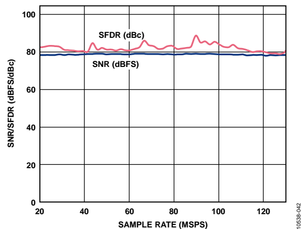
Figure 42. SNR/SFDR vs. Sample Rate, f_{IN} = 64 MHz, Clock Divider = 4, V_{REF} = 1.3 V
