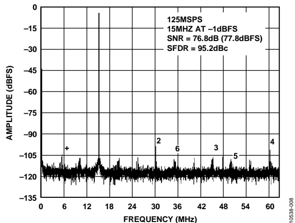
Figure 8. Single-Tone 16k FFT with f_{IN} = 15\text{ MHz} , f_{SAMPLE} = 125\text{ MSPS} , V_{REF} = 1.0\text{ V}
