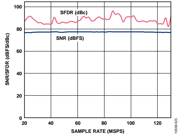
Figure 23. SNR/SFDR vs. Sample Rate, f_{IN} = 64 MHz, Clock Divider = 4, V_{REF} = 1.0 V
