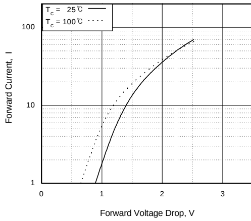
Fig 18. Forward Characteristics
