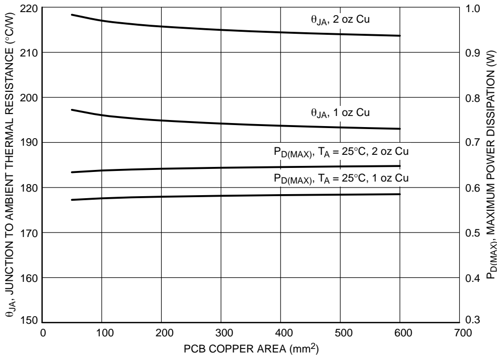
Figure 51. θ JA and P D(MAX) vs. Copper Area (XDFN4)
