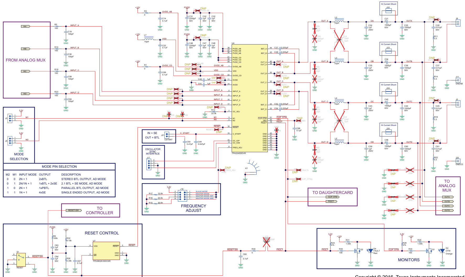
Figure 8. TPA3245EVM Schematic 2
