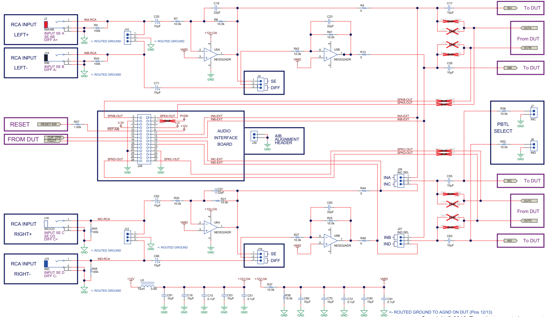
Figure 7. TPA3245EVM Schematic 1
