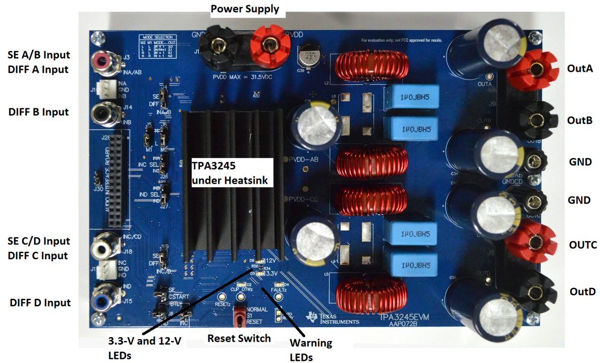
Figure 2. TPA3245EVM Connections
