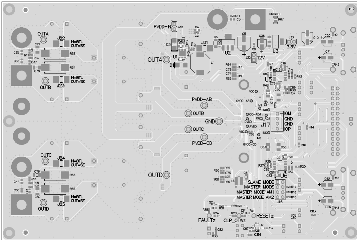
Figure 5. TPA3245EVM Bottom Composite Assembly
