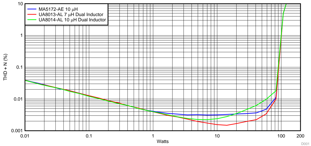
Figure 3. TPA3245EVM THD + N vs Output Power 30 V, BTL 4 \Omega , 600 kHz
