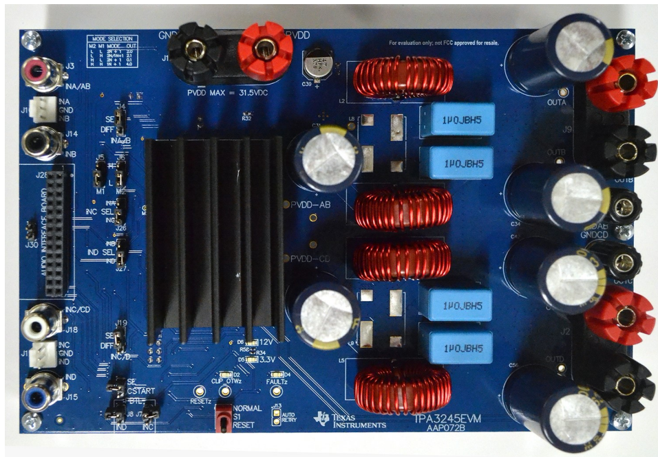
Figure 1. TPA3245EVM
