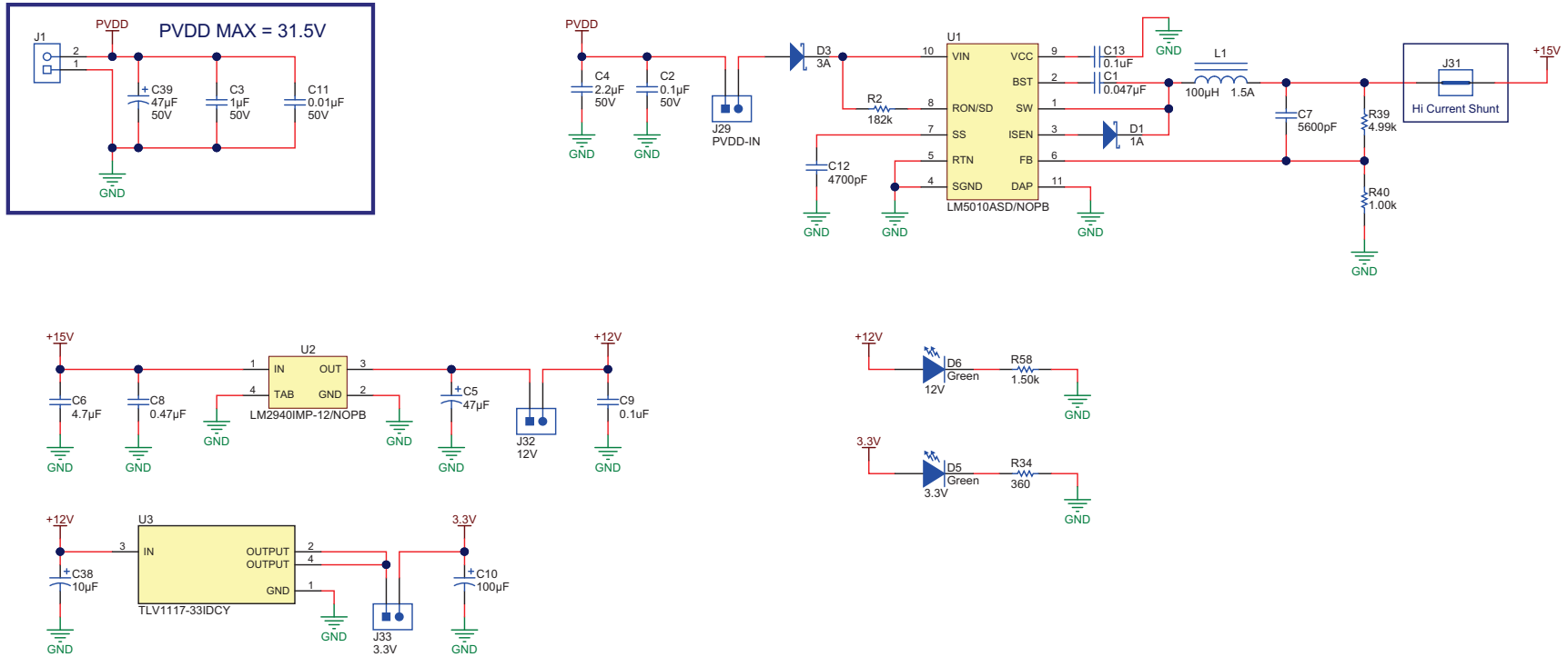
Figure 9. TPA3245EVM Schematic 3
