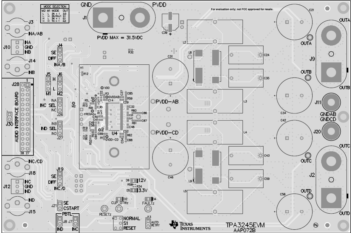
Figure 4. TPA3245EVM Top Composite Assembly
