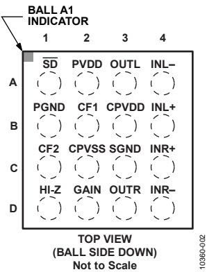
Figure 2. Pin Configuration
