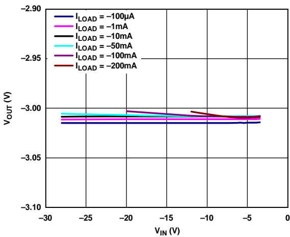
Figure 11. Output Voltage ( V_{OUT} ) vs. Input Voltage ( V_{IN} )
