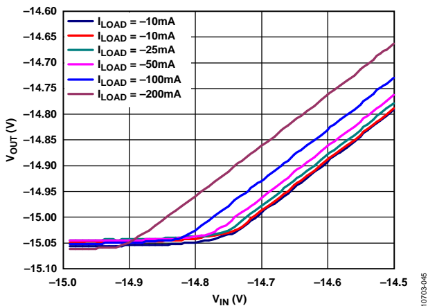
Figure 47. Output Voltage ( V_{OUT} ) vs. Input Voltage ( V_{IN} ) in Dropout, Adjustable Output Voltage, V_{OUT} = -15 V
