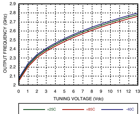
Divide-by-4 Frequency vs. Tuning Voltage
