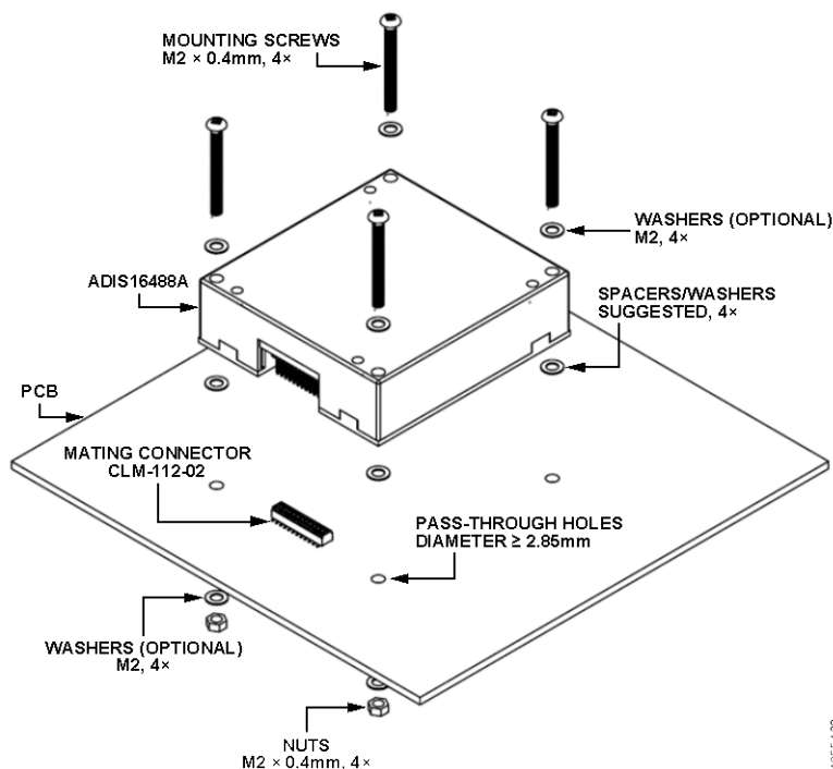
Figure 26. Mounting Example
