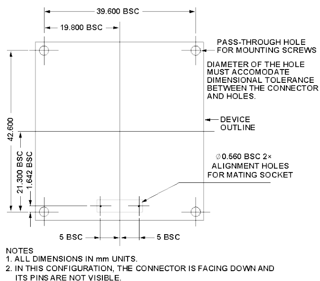
Figure 27. Suggested PCB Layout Pattern, Connector Down
