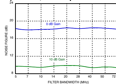
Figure 6. Noise Figure, 1 kΩ Source Impedance, 1 kΩ Impedance Selected [2]
