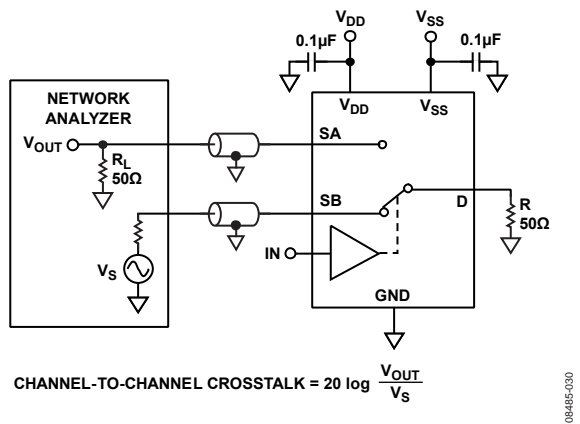
Figure 30. Channel-to-Channel Crosstalk
