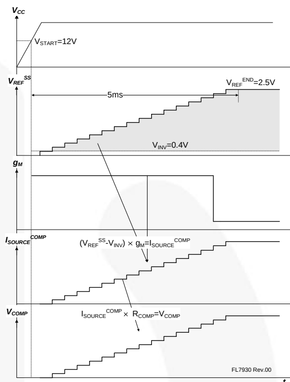
Figure 36. Soft-Start Sequence
