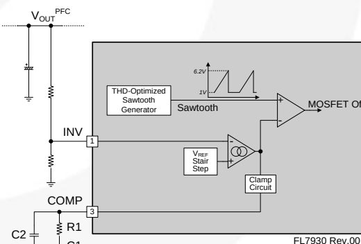
Figure 32. Control Circuit
