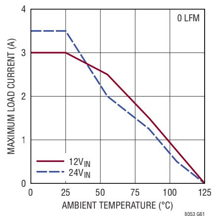
Derating, V_{OUT} = -8\text{V} , BIAS Open, DC1934A Demo Board
