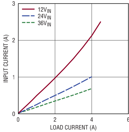
Input vs Load Current V_{OUT} = -5\text{V} , BIAS OPEN
