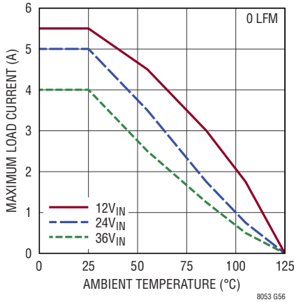
Derating, V_{OUT} = 8\text{V} , BIAS = 5V, DC1934A Demo Board
