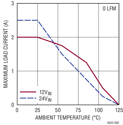
Derating, V_{OUT} = -12\text{V} , BIAS Open, DC1934A Demo Board
