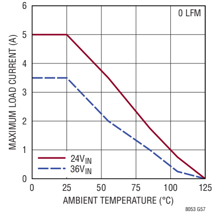
Derating, V_{OUT} = 12\text{V} , BIAS = 5V, DC1934A Demo Board
