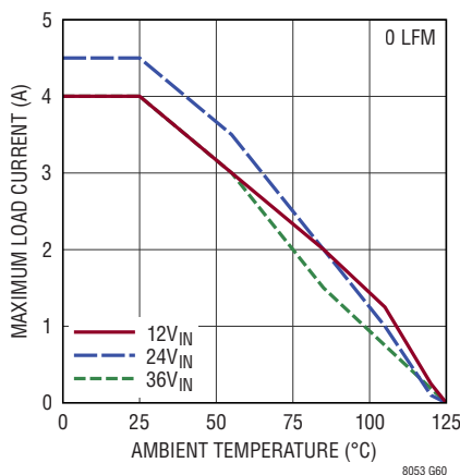
Derating, V_{OUT} = -5\text{V} , BIAS Open, DC1934A Demo Board
