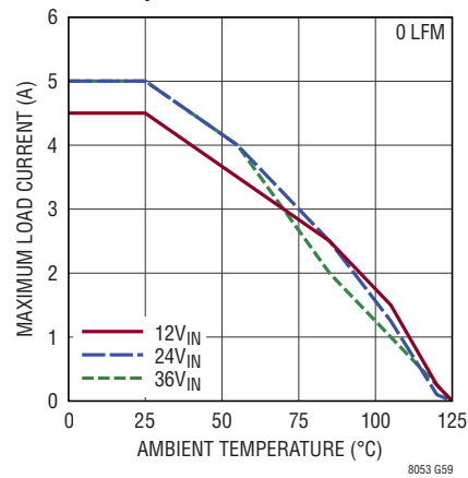
Derating, V_{OUT} = -3.3\text{V} , BIAS Open, DC1934A Demo Board
