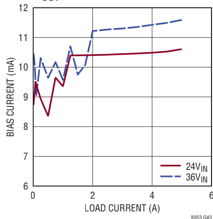
BIAS Current vs Load Current V_{OUT} = 15V , BIAS = 5V
