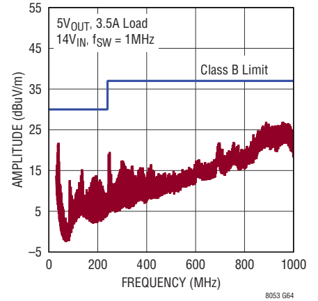
CISPR32 Class B Emissions DC1934A Demo Board, No EMI Filter ( C_{10} = 0.1\mu\text{F} , Short L1, Open C7)
