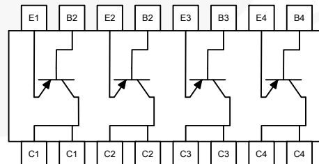
Figure 6. MMPQ2907A Internal Connections
