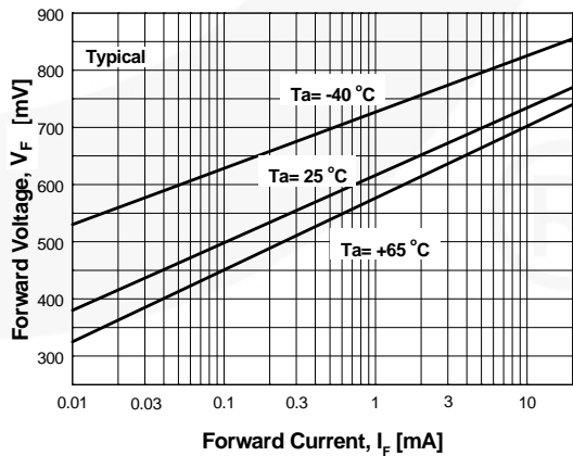
Figure 6. Forward Voltage vs. Ambient Temperature V_F - 0.01 - 20 mA (-40 to +65 ^\circ\text{C} )
