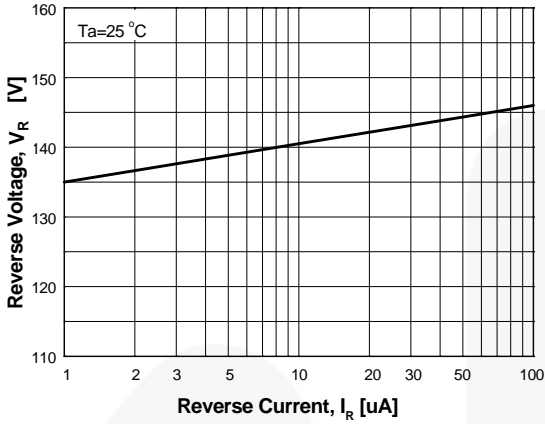
Figure 1. Reverse Voltage vs. Reverse Current V_R - 1.0 to 100 \mu\text{A}
