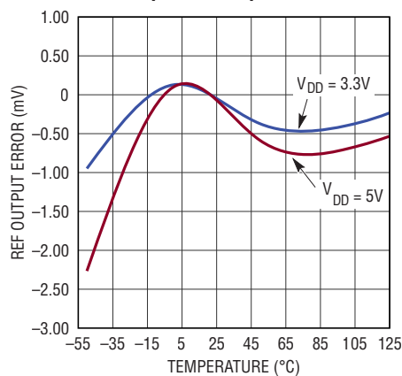
REF Output vs Temperature
