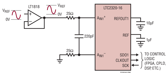
Figure 6. Pseudo-Differential Unipolar Application Circuit
