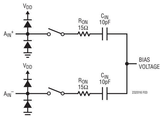
Figure 3. The Equivalent Circuit for the Differential Analog Input of the LTC2320-16
