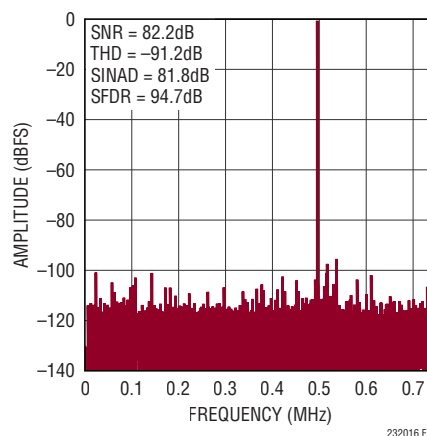
Figure 16. 32k Point FFT of the LTC2320-16
