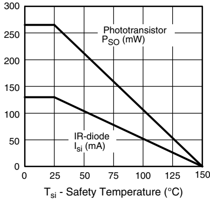
Fig. 4 - Derating Diagram
