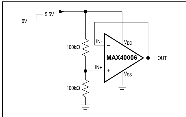
Figure 3. Power-Up Test Configuration
