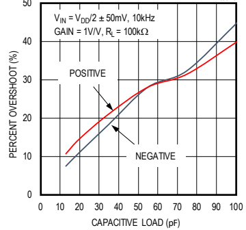
PERCENT OVERSHOOT vs. CAPACITIVE LOAD
