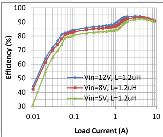
Figure 7. FAN2306 Efficiency vs. Load Current with V_{OUT}=1.2\text{ V} and f_{SW}=500\text{ kHz}
