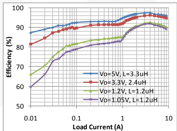
Figure 8. FAN2306M Efficiency vs. Load Current with V_{IN}=12\text{ V} and f_{SW}=500\text{ kHz}
