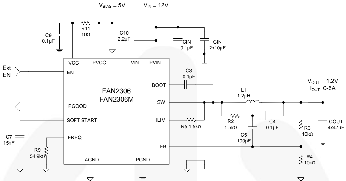
Figure 1. Typical Application
