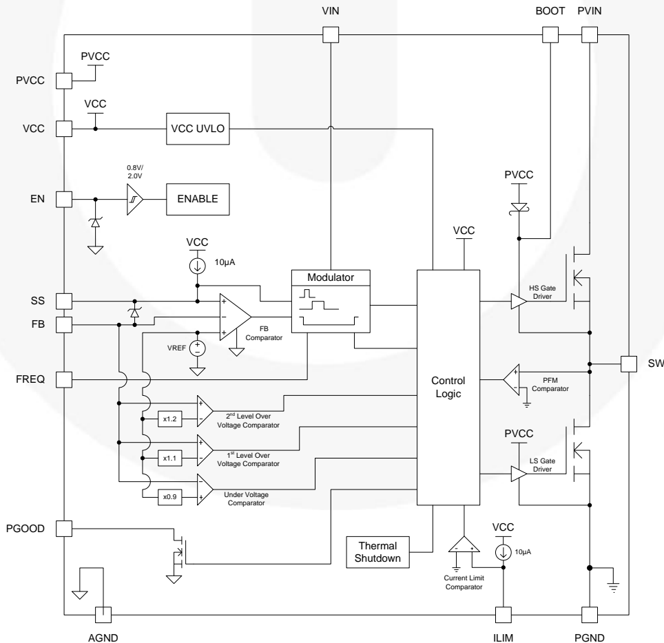
Figure 2. Block Diagram
