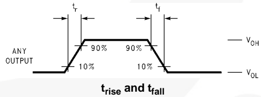
Figure 2. Waveforms
