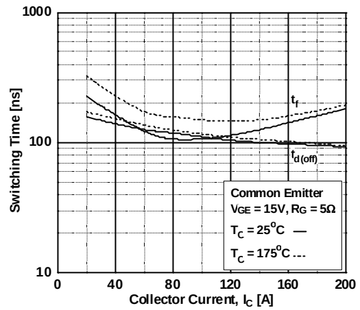
Figure 16. Turn-off Charateriztics vs. Collector Current
