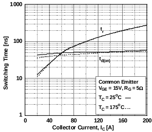
Figure 15. Turn-on Charateriztics vs. Collector Current
