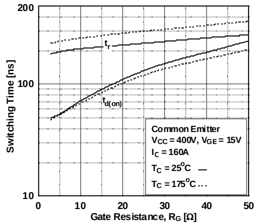
Figure 13. Turn-on Charateriztics vs. Gate
