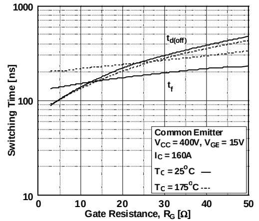
Figure 14. Turn-off Charateriztics vs. Gate
