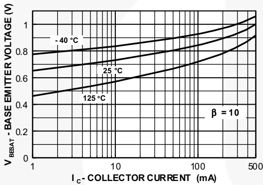
Figure 9. Base-Emmitter Saturation Voltage vs. Collector Current
