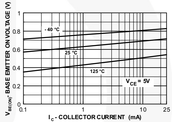
Figure 10. Base-Emmitter On Voltage vs. Collector Current
