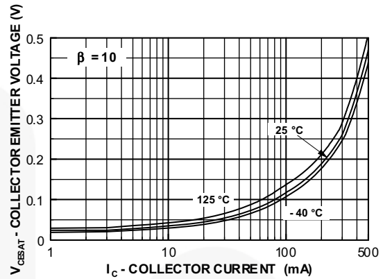
Figure 8. Collector-Emmitter Saturation Voltage vs. Collector Current
