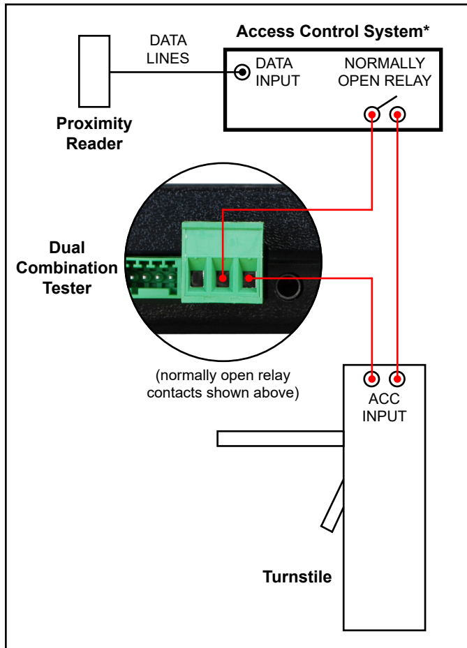
Figure 5. Wiring the Dual Combination Tester to an Access Control System
