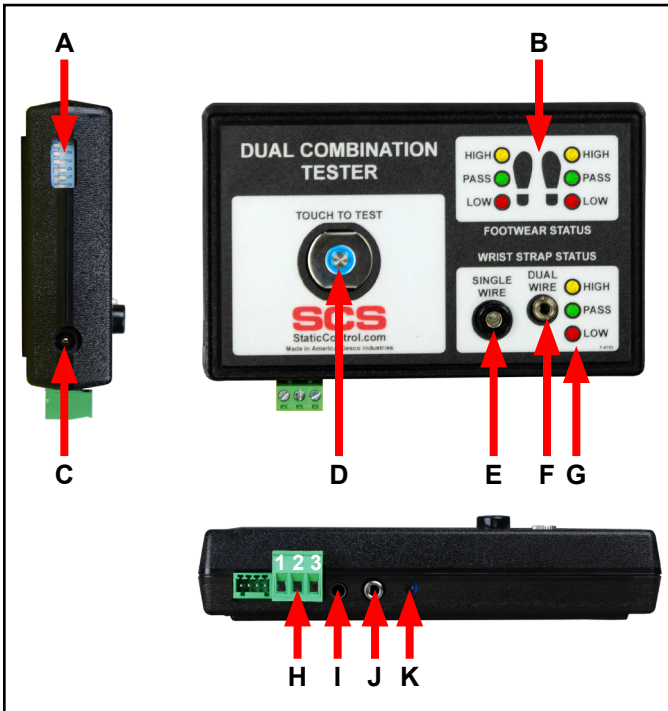
Figure 3. Dual Combination Tester features and components
