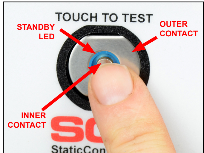
Figure 6. Steady-State Test Switch features and components
