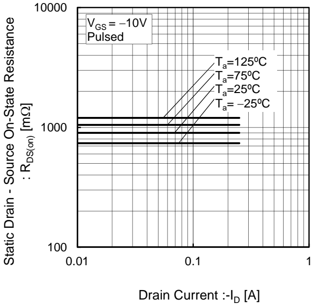
Fig.12 Static Drain-Source On-State Resistance vs. Drain Current(II)
