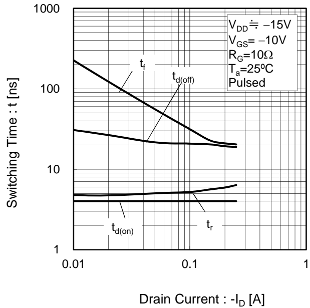
Fig.16 Switching Characteristics
