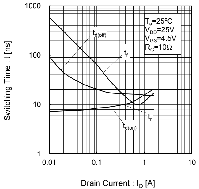
Fig.19 Switching Characteristics
