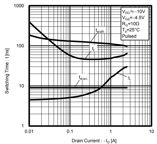
Fig.12 Switching Characteristics
