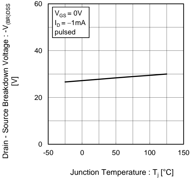
Fig.5 Breakdown Voltage vs. Junction Temperature
